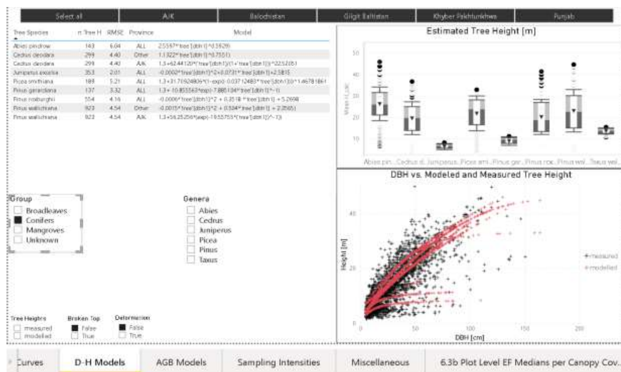
Figure 13: Visual assessment of D-H models for conifers in PBI analysis.
